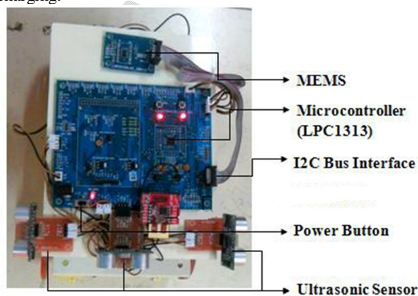
Figure.13. Prototype of the Robot
