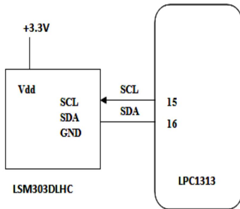
Figure.10. Interfacing diagram of MEMS with microcontroller
