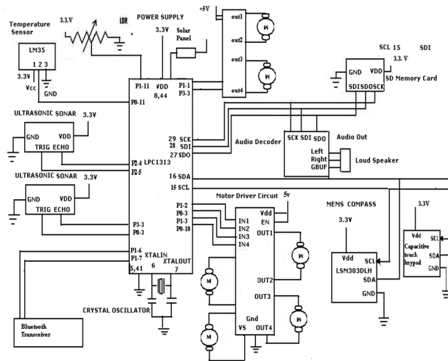
Figure1. Circuit Diagram
