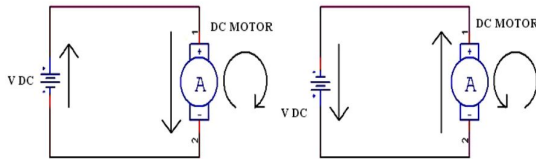
Figure.6. Motor Direction Control
