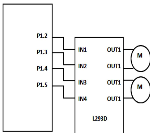
Figure.12. Interfacing diagram for motor control with Microcontroller
