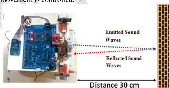
Figure 4. In-front Obstacle Detection
