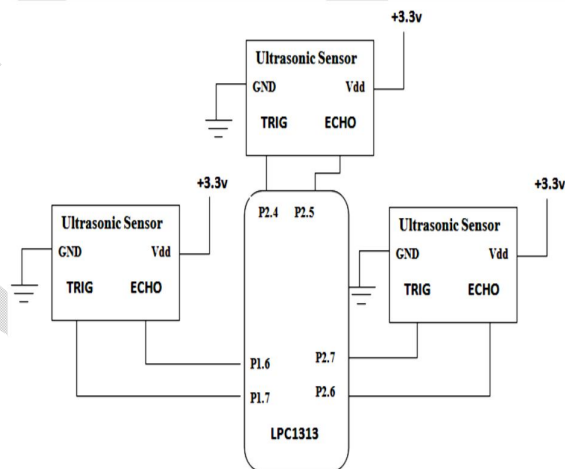
Figure 8. Interfacing diagram for Ultrasonic sensor with Microcontroller
